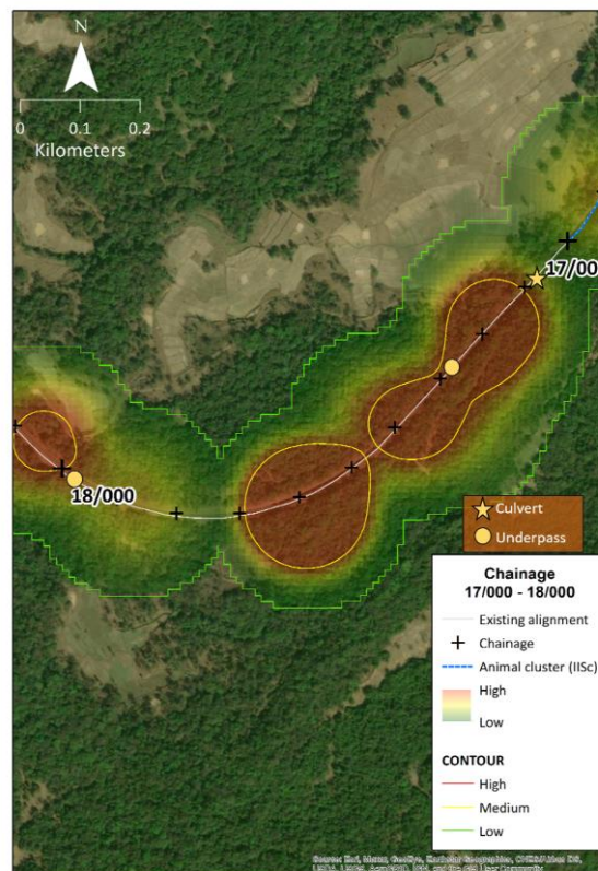
Figure 33: Locations of mitigation measures on chainage 17/000 – 18/000 to be constructed on existing and proposed railway track
