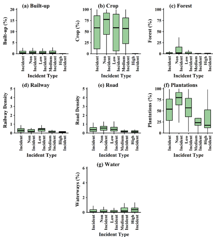
Figure 1.15: Comparison of ecological and anthropogenic variables across different incident types and non-incident villages of Kerala in relation to Human-Elephant Conflict
